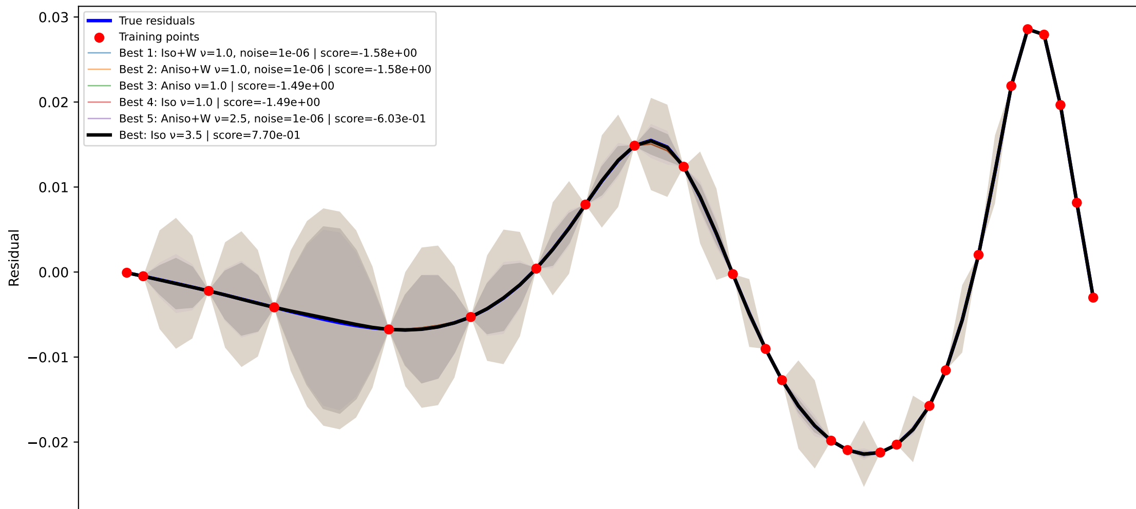
GPR kernel comparison node=19 RMSE=4.918e-05, train RMSE=1.997e-11
